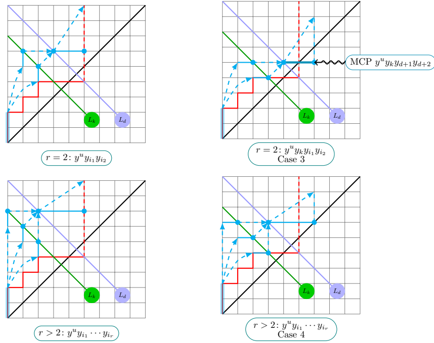
Figure 2: On the left are the path of monomials y^\beta for \beta \in P_\alpha^{(k)} . On the right are the path of the terms in Equation (3) for r > 1
