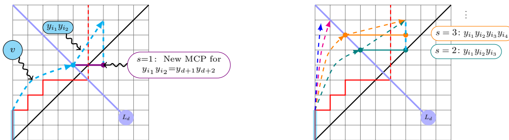
Figure 1: On the left is Case 1 and on the right is Case 2
