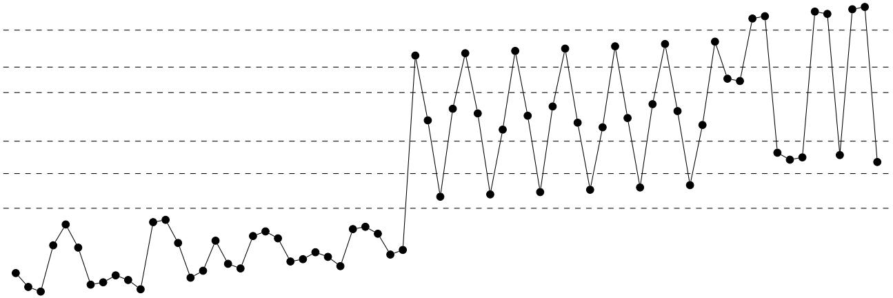
Figure 2: A bicrucial permutation of length 72 constructed as in the proof of Theorem 3.2. The dashed lines divide \{0, \dots, 71\} into the 7 different regions used in the construction.
