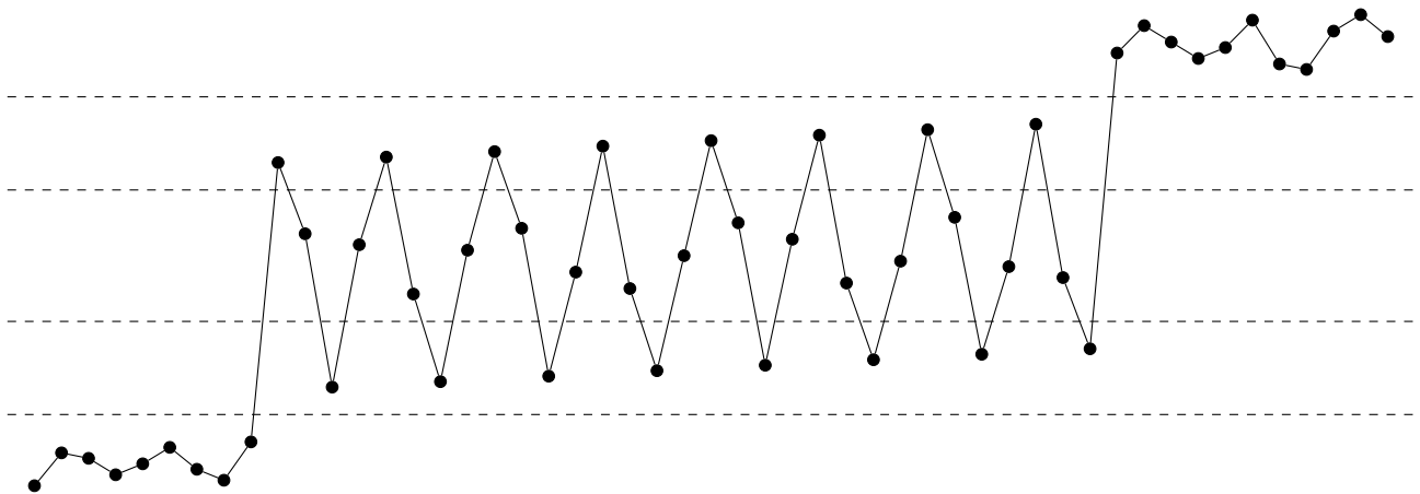
Figure 1: A bicrucial permutation of length 51 constructed as in the proof of Theorem 3.1. The dashed lines separate the different regions.
