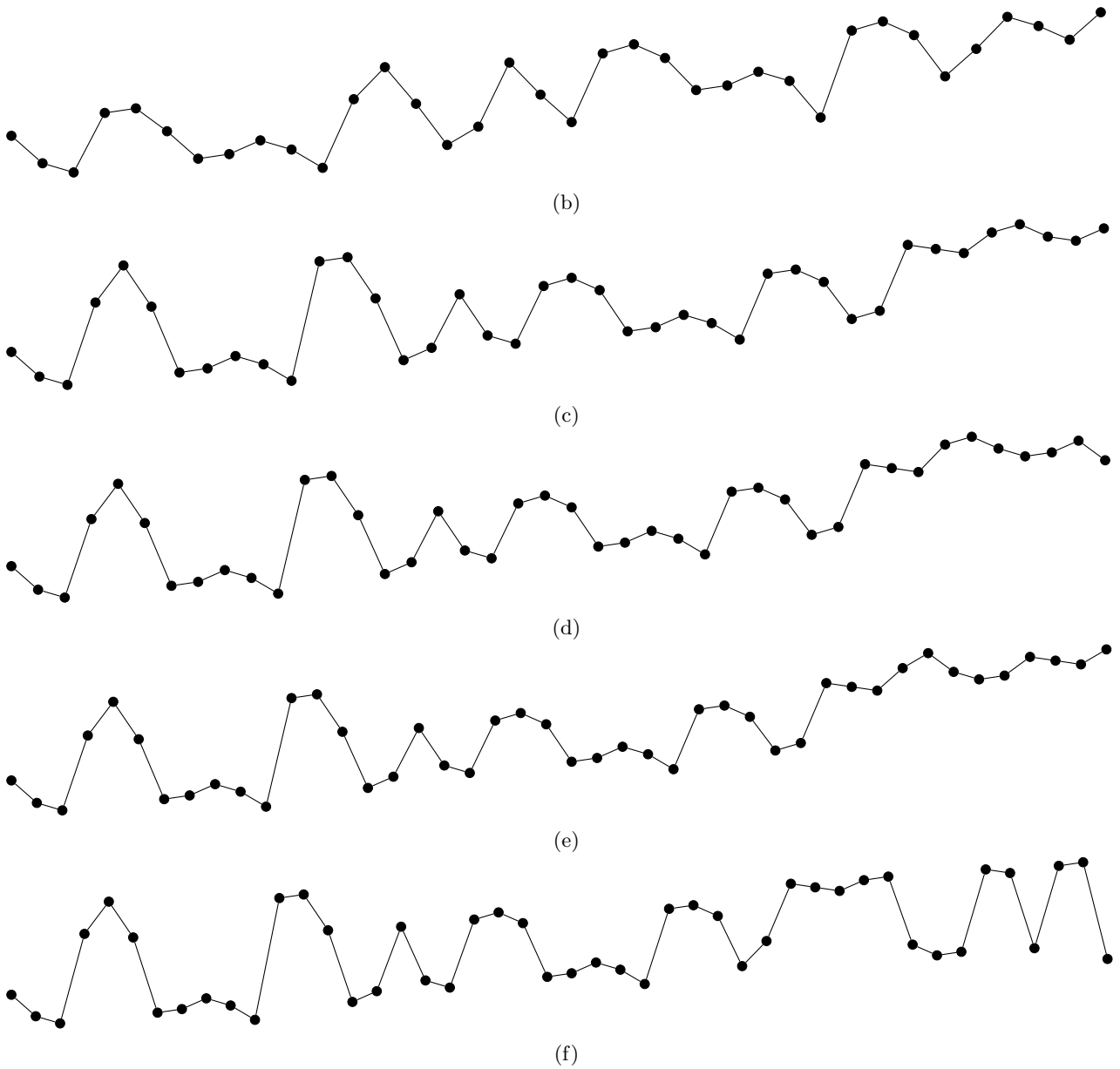
Figure 4: Bicrucial permutations of lengths 34, 36, 40, 42, 44 and 46 respectively.
