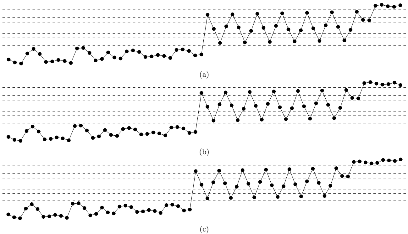
Figure 3: Bicrucial permutations of length 64, 66 and 68 constructed as in the proof of Theorem 3.2. The dashed lines divide \{0, \dots, n - 1\} into the 7 different regions used in the construction.
