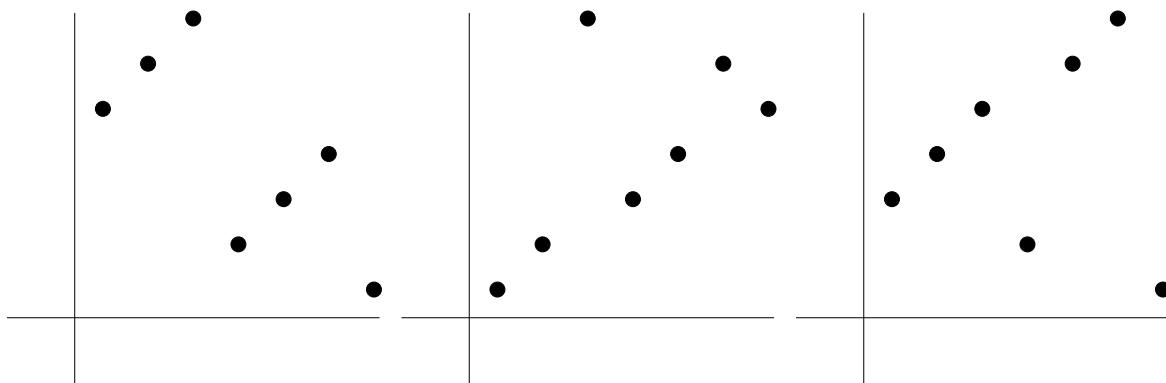
(a) The form of a permutation in B_n(132, 213) . (b) The form of a permutation in B_n(213, 231) . (c) The form of a permutation in B_n(132, 312) .
