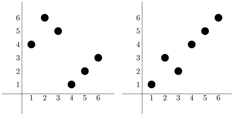
(a) The graph of the skew sum described in Example 2.1. (b) The graph of the direct sum described in Example 2.2.
